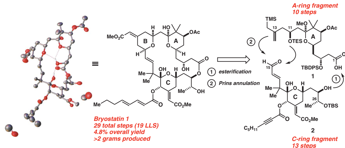
Fig. 1. Retrosynthetic analysis of bryostatin 1, and its crystal structure (with bound methanol) determined by x-ray diffraction.
