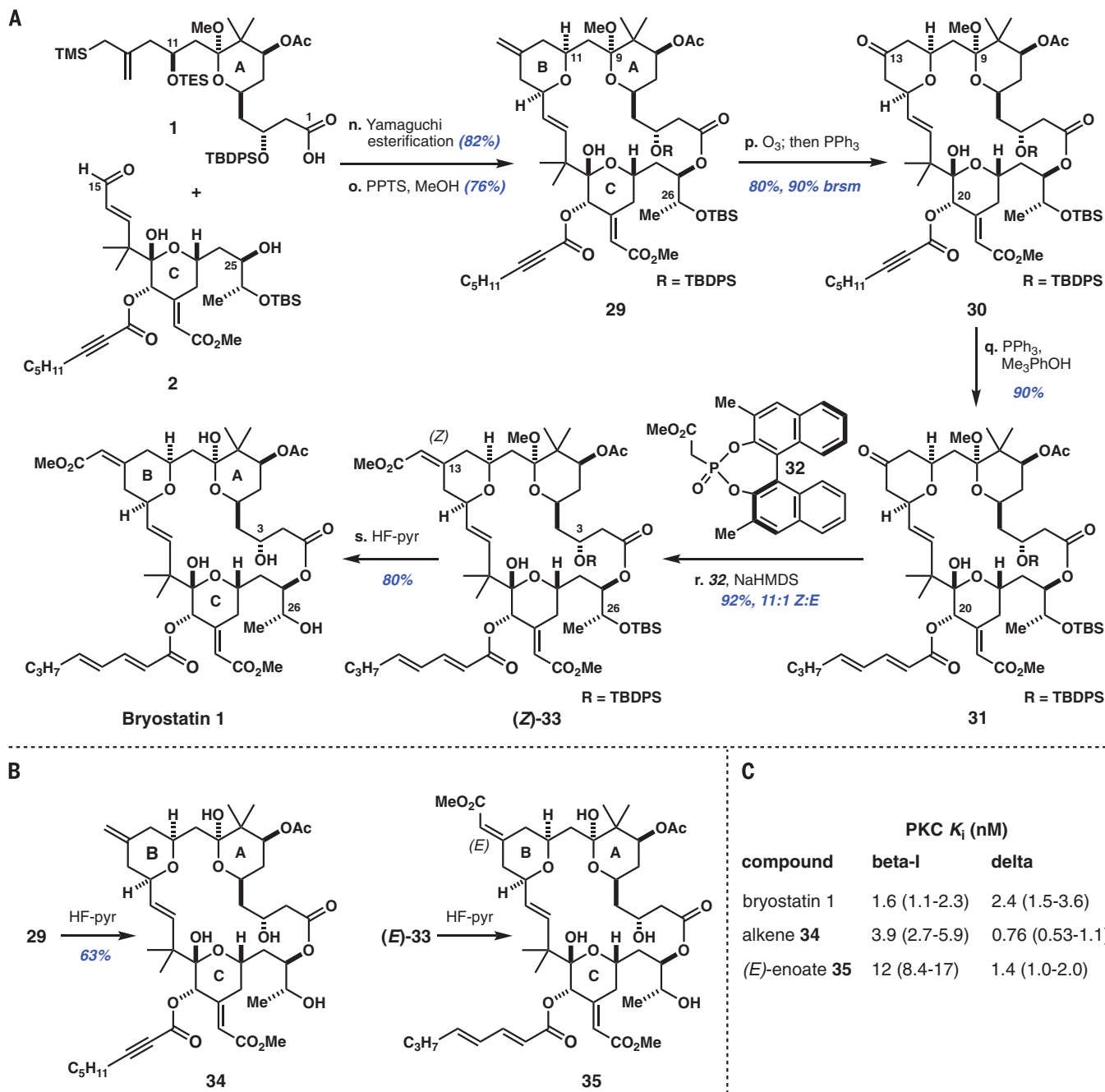
Fig. 4. Completion of bryostatin 1 synthesis and one-step diversifications toward analog compounds. (A) Reaction sequence for bryostatin 1; (B) synthesis of derivatives 34 and 35 ; (C) characteristics of 34 and 35 versus bryostatin 1. Reagents and conditions: n. Acid 1 (1 equiv), 2,4,6-trichlorobenzoyl chloride (1.8 equiv), \text{Et}_3\text{N} (6 equiv), toluene; then alcohol 2 (1 equiv), DMAP (3 equiv). o. PPTS (30 mol %), 50:1 MeOH/ \text{CH}(\text{OMe})_3 . p. Ozone (~1.9 equiv), MeOH/ \text{CH}_2\text{Cl}_2 , -78^\circ\text{C} ; then triphenylphosphine ( \text{Ph}_3\text{P} ) (2 equiv), -78^\circ\text{C} to room temperature. q. \text{Ph}_3\text{P} (5 equiv), 2,4,6-trimethylphenol (5 equiv), benzene. r. Phosphonate 32 (14 equiv), sodium hexamethyldisilazide (NaHMDS) (13 equiv), THF, -78^\circ to 4^\circ\text{C} . s. 1:2:2 HF-pyridine/pyridine/THF, 40^\circ\text{C} ; then \text{H}_2\text{O} , 40^\circ\text{C} . See supplementary materials for PKC binding assay protocol. Error ranges in parentheses indicate 95% confidence intervals from nonlinear regression analysis.
