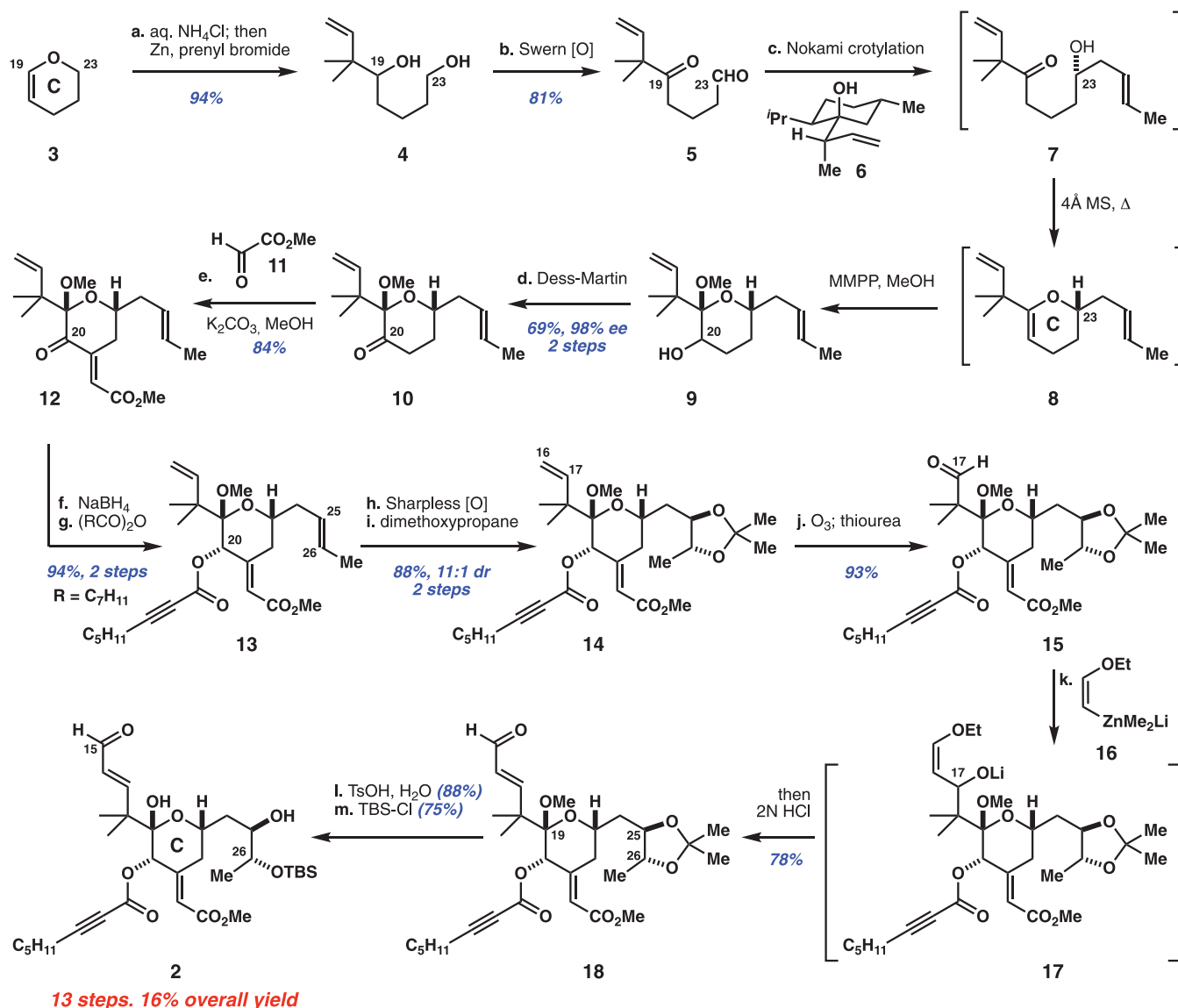
Fig. 2. Reaction sequence for the C-ring subunit, 2 . Reagents and conditions: a. \text{NH}_4\text{Cl} , \text{H}_2\text{O} ; then zinc powder (3.4 equiv), prenyl bromide (1.7 equiv), tetrahydrofuran (THF). b. Oxalyl chloride (3 equiv), dimethyl sulfoxide (DMSO) (4 equiv), \text{CH}_2\text{Cl}_2 , -78^\circ\text{C} ; then 4 ; then \text{Et}_3\text{N} (8 equiv), -78^\circ\text{C} to -30^\circ\text{C} . c. Reagent 6 (2 equiv), p -toluenesulfonic acid ( p - \text{TsOH}\cdot\text{H}_2\text{O} ) (10 mol %), \text{CHCl}_3 ; then 4 Å molecular sieves, 70^\circ\text{C} ; then magnesium monoperoxyphthalate (MMPP) hexahydrate (0.45 equiv), \text{NaHCO}_3 (2 equiv), MeOH, 0^\circ\text{C} . d. Dess-Martin periodinane (1.5 equiv), pyridine (10 equiv), \text{CH}_2\text{Cl}_2 , 0^\circ\text{C} . e. Glyoxylate 11 (5 equiv), \text{K}_2\text{CO}_3 (5.5 equiv), 4.4:1 THF/MeOH. f. \text{CeCl}_3\cdot 7\text{H}_2\text{O} (0.5 equiv), \text{NaBH}_4 (2 equiv), MeOH, -50^\circ\text{C} . g. (\text{C}_7\text{H}_{11}\text{CO})_2\text{O} (3 equiv), 4-dimethylaminopyridine (DMAP) (1 equiv), \text{CH}_2\text{Cl}_2 , -20^\circ\text{C} to 0^\circ\text{C} . h. \text{K}_2\text{OsO}_2(\text{OH})_4 (1 mol %), dihydroquinidine 1,4-phthalazinediyl diether (DHQD) 2 PHAL (5 mol %), \text{K}_3\text{Fe}(\text{CN})_6 (3 equiv), \text{K}_2\text{CO}_3 (3 equiv), \text{MeSO}_2\text{NH}_2 (1 equiv), 1:1 t -BuOH/ \text{H}_2\text{O} , 0^\circ\text{C} . i. 2,2-Dimethoxypropane (4 equiv), PPTS (10 mol %), \text{CH}_2\text{Cl}_2 . j. Ozone (~1.8 equiv), \text{CH}_2\text{Cl}_2 , -78^\circ\text{C} ; then thiourea (10 equiv), i -PrOH, -78^\circ\text{C} to room temperature. k. Cis -1-bromo-2-ethoxyethylene (8 equiv), t -BuLi (16 equiv), \text{Me}_2\text{Zn} (8.8 equiv), \text{Et}_2\text{O} , -78^\circ\text{C} ; then aldehyde 15 ; then 1M HCl (64 equiv). l. p - \text{TsOH}\cdot\text{H}_2\text{O} (1 equiv), 4:1 MeCN/ \text{H}_2\text{O} , room temperature to 45^\circ\text{C} . m. t -Butyldimethylsilyl chloride (TBS-Cl) (1.5 equiv), imidazole (2 equiv), N,N -dimethylformamide (DMF). Me, methyl; Et, ethyl; Bu, butyl.
